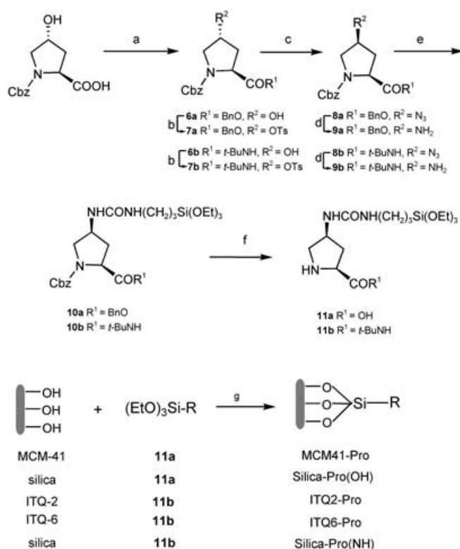
Scheme 2. Reagents and conditions: a) (i) Et 3 N, ClCOOEt, THF, 0 °C, 30 min; (ii) BnOH, reflux, 24 h, 70% for 6a ; t -BuNH 2 , reflux, 2 h, 89.5% for 6b ; b) TsCl, Py, r.t., 48 h, 80% for 7a ; 100% for 7b ; c) NaN 3 , DMF:water, 70 °C, 48 h, 80% for 8a ; 100% for 8b ; d) Pd/C (5%), AcOEt, 20 h, 89% for 9a ; 97% for 9b ; e) (EtO) 3 Si(CH 2 ) 3 NCO, CH 2 Cl 2 , r.t., 18 h, 100%; f) Pd/C, cyclohexene, EtOH, r.t., 15 min for 11a ; 1 h for 11b , 100%; g) toluene, reflux, 18 h.
