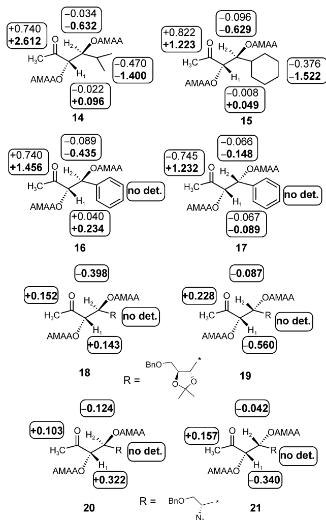
Figure 2. \Delta\delta^{RS} values for diester derivatives of aldol products. Plain and bold numbers correspond to values from MPA and 9-AMA, respectively.
