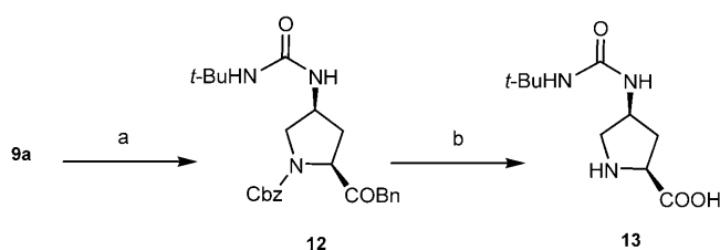
Scheme 3. Reagents and conditions: a) t -BuNCO, CH 2 Cl 2 , r.t., 1 h, 100%; b) Pd/C, cyclohexene, EtOH, reflux, 15 min, 100%.
