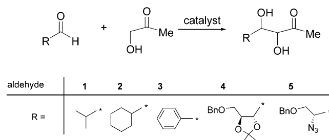
Scheme 1. Aldol condensation between hydroxyacetone and different aldehydes catalyzed by L-proline or mesoporous material.
