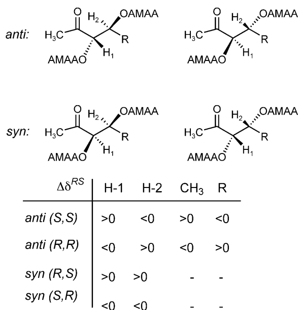
Figure 1. Diagnostic \Delta\delta^{RS} signs for the four possible stereoisomers.
